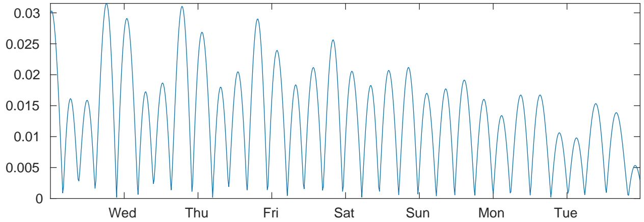
Surface tidal current speed, knots
