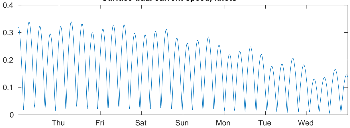
Surface tidal current speed, knots
